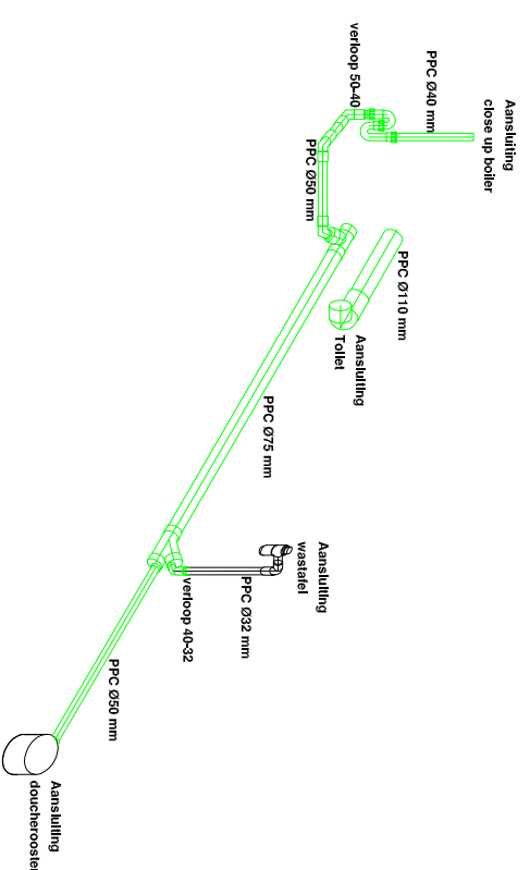
Riolering set
